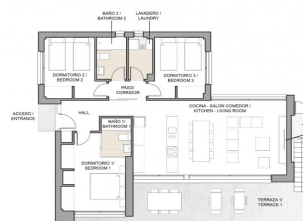
PLANTA BAJA / GROUND FLOOR
